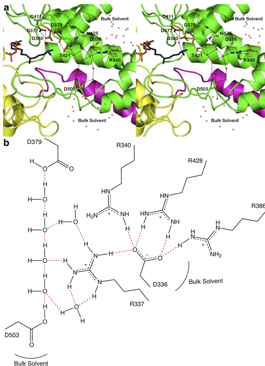
Fig. 4. (a) Cut-away view of the CPS active site showing solvent channels leading to general acid D379. One channel leads to D503 and the solvent-exposed surface of the \beta domain (green) near the interface with the \gamma domain (yellow); the other channel leads to D336–R340, which are exposed to bulk solvent at the interface of the \alpha (blue) and \beta domains. These channels are distinct from the main active site cleft, which opens to the left in this view. (b) Molecular scheme showing hydrogen bond interactions linking general acid D379 with bulk solvent through the two polar solvent channels shown in (a). For clarity, R337, R386, and R428 are omitted from the view in (a) but are shown here to emphasize the highly polar nature of the hydrogen bond networks with D379.
