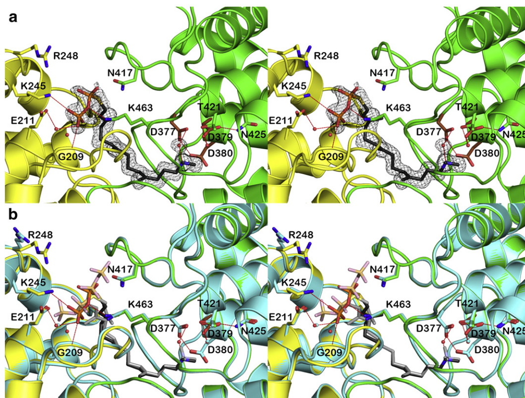
Fig. 3. (a) Simulated annealing omit map (contoured at 4.0 \sigma ) of the CPS-1 complex at 1.55 Å resolution. Atoms are color-coded as follows: C = green ( \beta domain), brown (DXDD general acid motif in the \beta domain), or yellow ( \gamma domain), N = blue, O = red, P = orange, S = yellow; selected water molecules are shown as small red spheres, and hydrogen bond interactions are indicated by dash red lines. (b) Superposition of the 1.55 Å-resolution structure of the CPS-1 complex color-coded as in (a) with the 2.25 Å-resolution structure (all atoms cyan).
